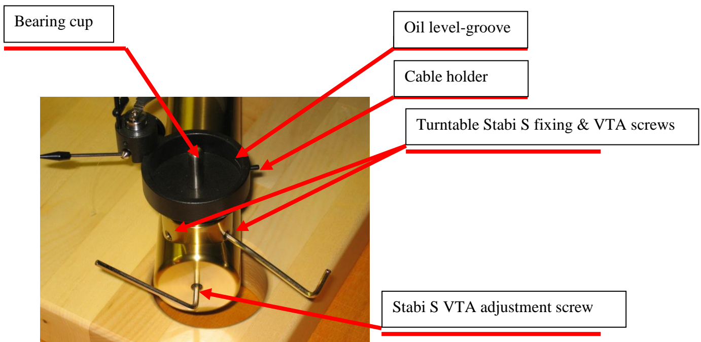
Fig. 3 . The bearing base with cable holder in its brass pillar on Stabi S
