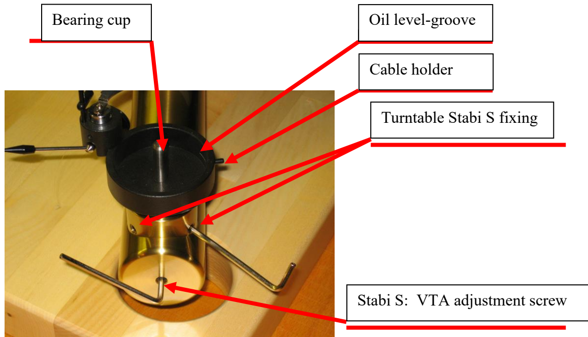
Fig. 3. The bearing base with cable holder in its brass pillar on Stabi S.
